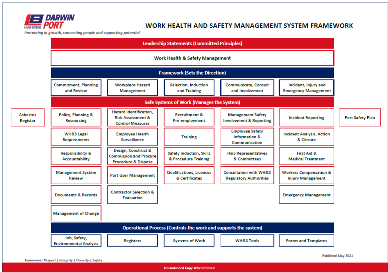
FIGURE 4 – SMS Framework
